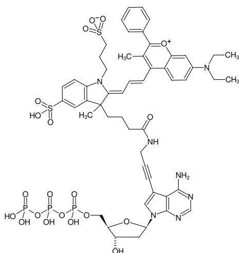
Structural formula of 7-Propargylamino-7-deaza-dATP-DYQ-661
