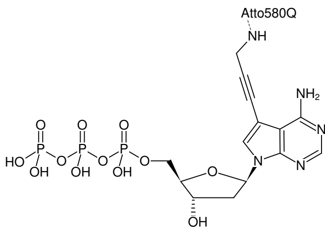
Structural formula of 7-Propargylamino-7-deaza-dATP-ATTO-580Q
