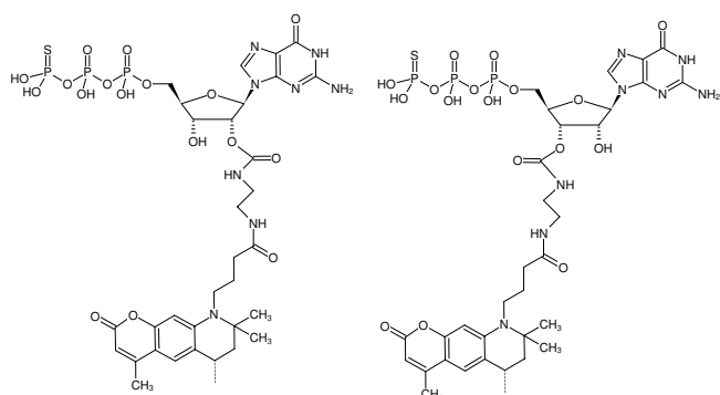
Structural formula of EDA-GTPyS-ATTO-390
