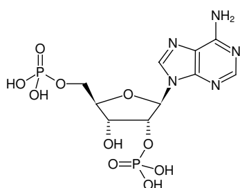
Structural formula of Adenosine-2',5'-bisphosphate
