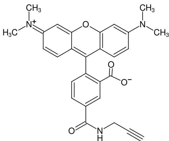
Structural formula of 5-TAMRA-Alkyne
